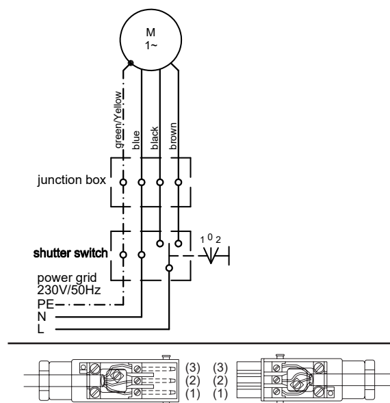
Fig. 5 Circuit diagram RolTop 230 V / 50 Hz and wiring when used with Hirschmann plug STAS 3
